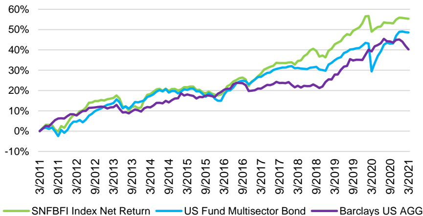
Cumulative Returns 1
